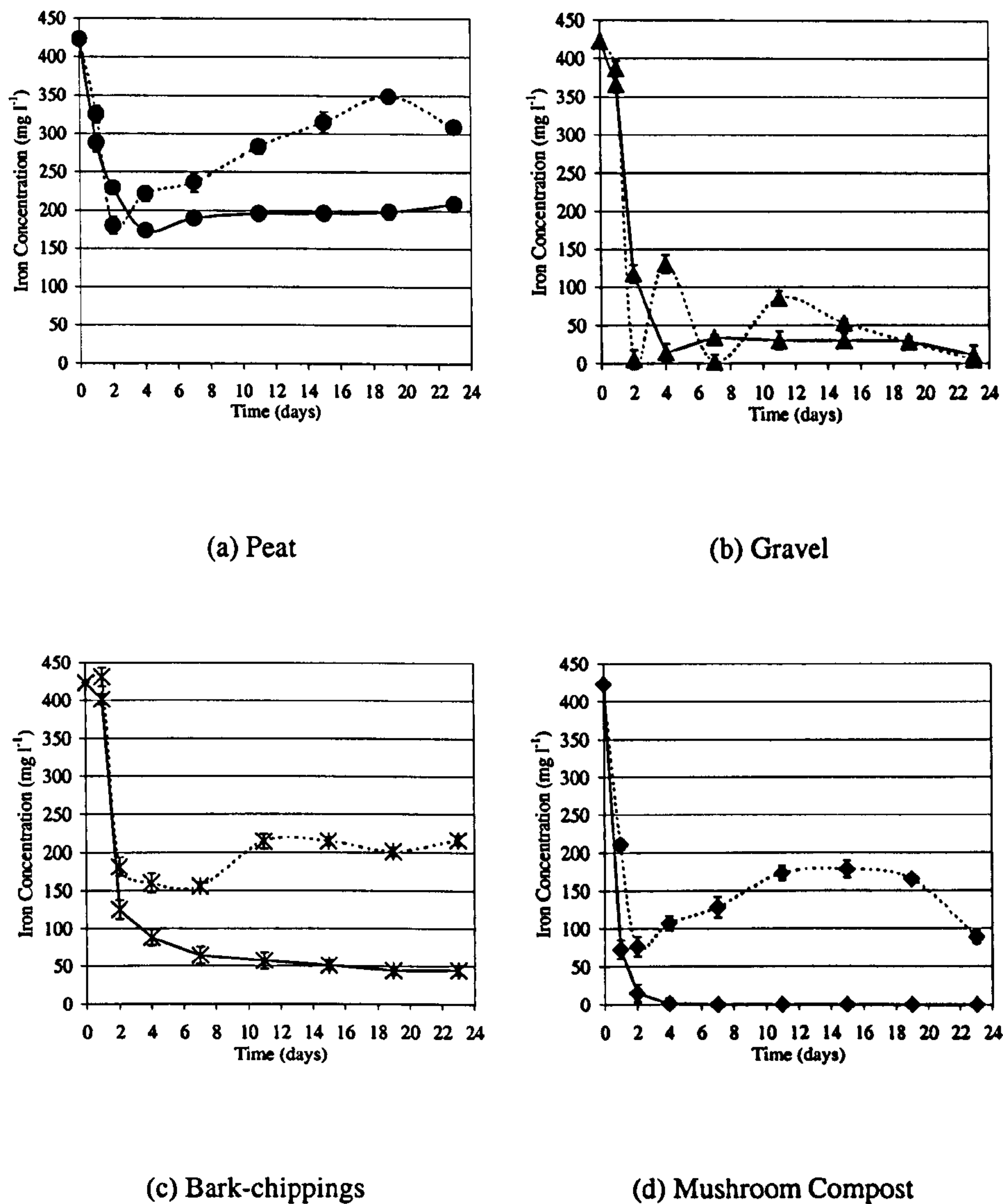
Figure 4.3: The effect of soil type and planting on interstitial water dissolved iron concentrations in microcosms treating waters obtained from Mona adit (mean \pm s.e., n=4). Planted microcosms represented by dotted line, unplanted microcosms represented by solid line.
