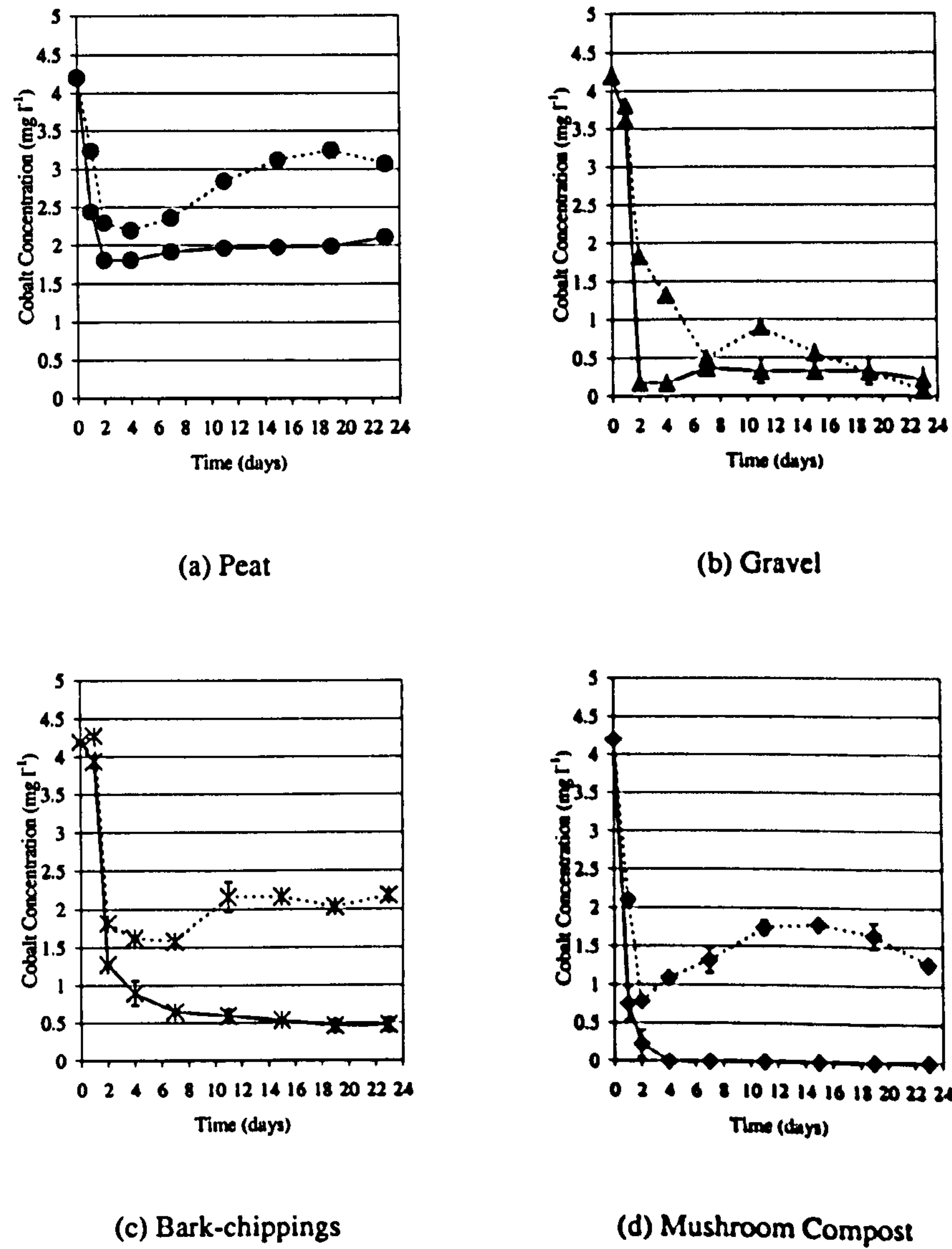
Figure 6.6: The effect of soil type and planting on interstitial water cobalt concentrations in microcosms treating Mona mine waters (mean \pm s.e., n=4). Planted microcosms represented by dotted line, unplanted microcosms represented by solid line.
