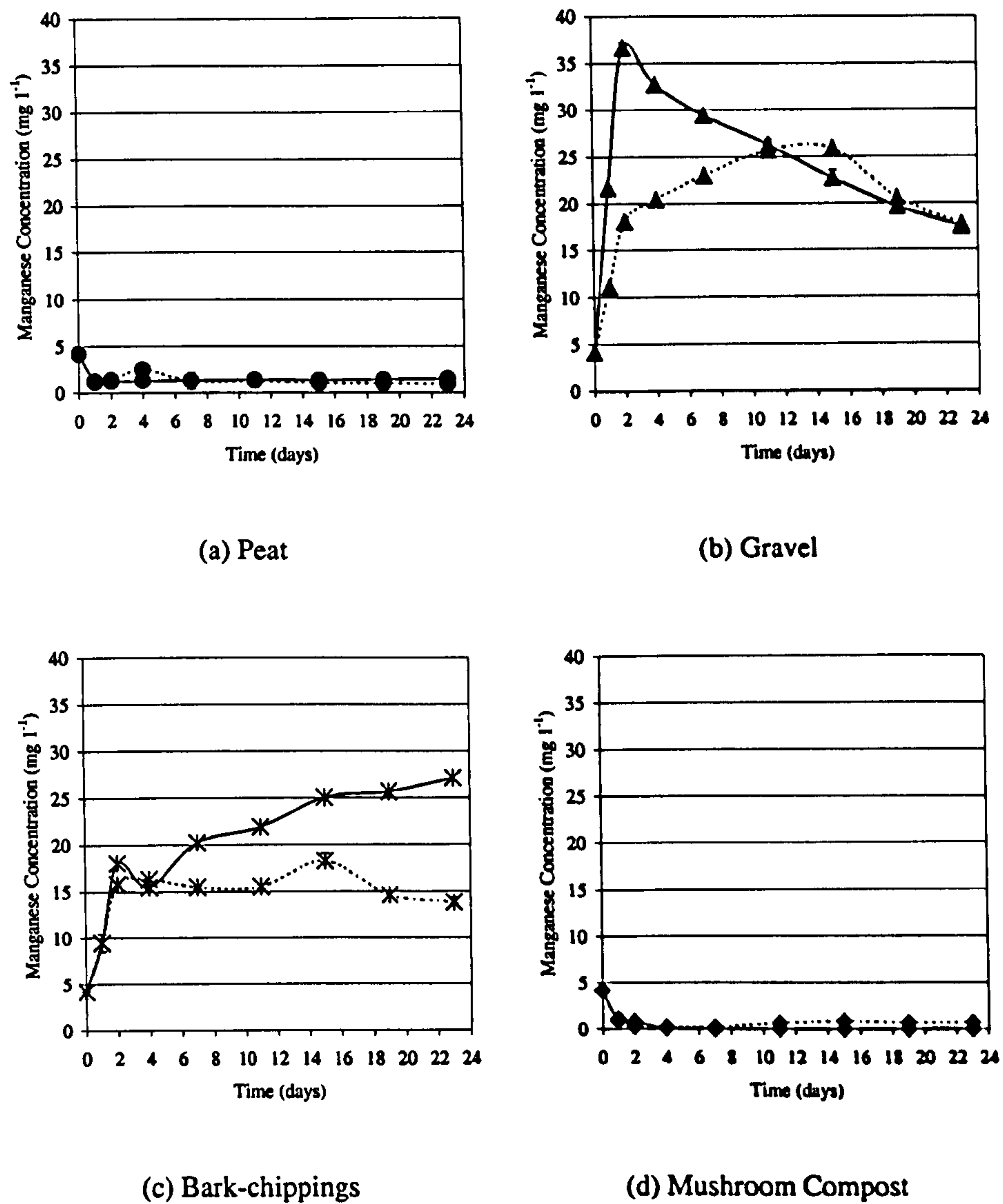
Figure 6.2: The effect of soil type and planting on interstitial water manganese concentrations in microcosms treating Ynysarwed mine waters. Mean \pm s.e., n=4 . Planted microcosms represented by dotted line, unplanted microcosms represented by solid line.
