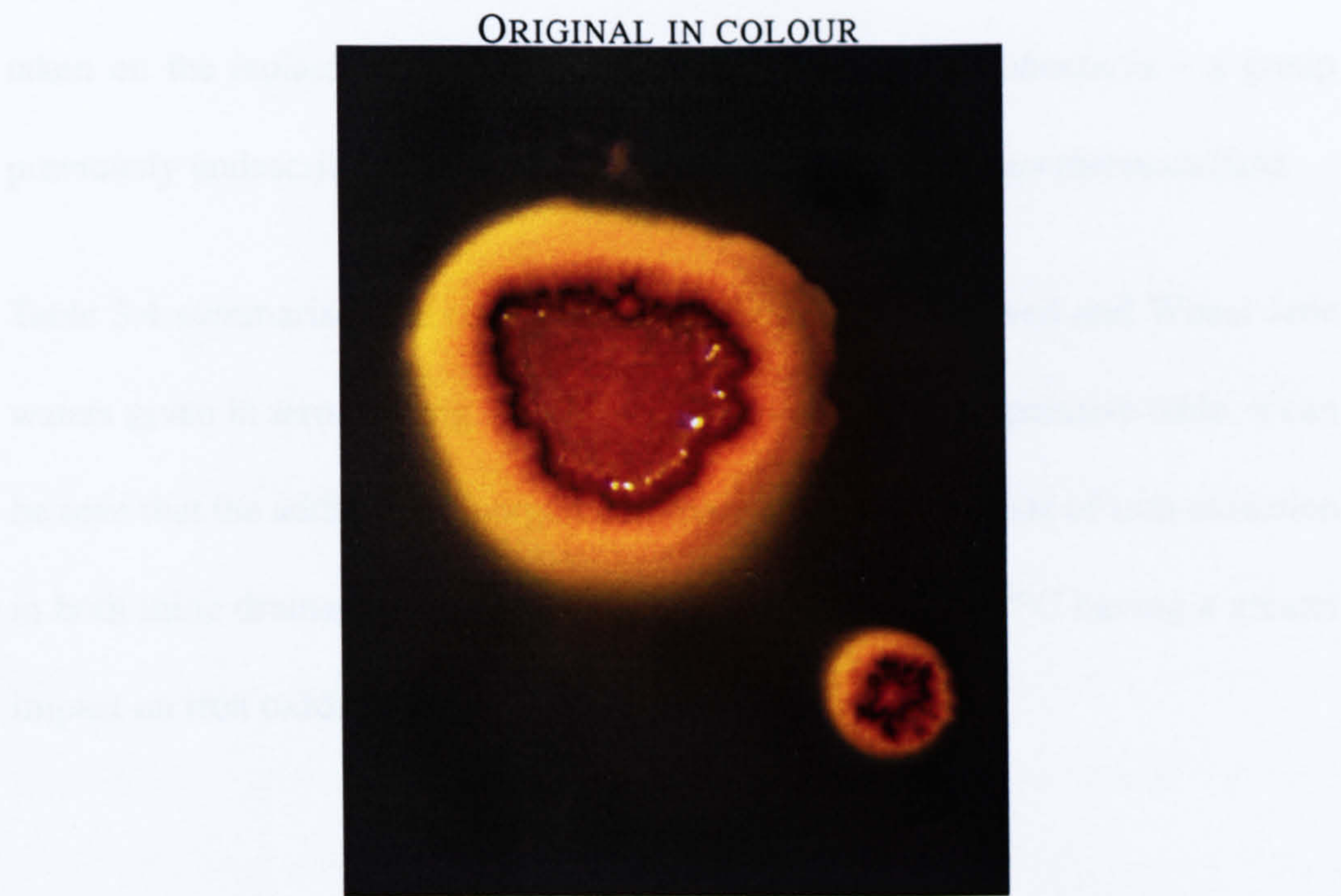
Figure 3.13: Both new isolates (x25), as isolated on Fe/thio plates.
