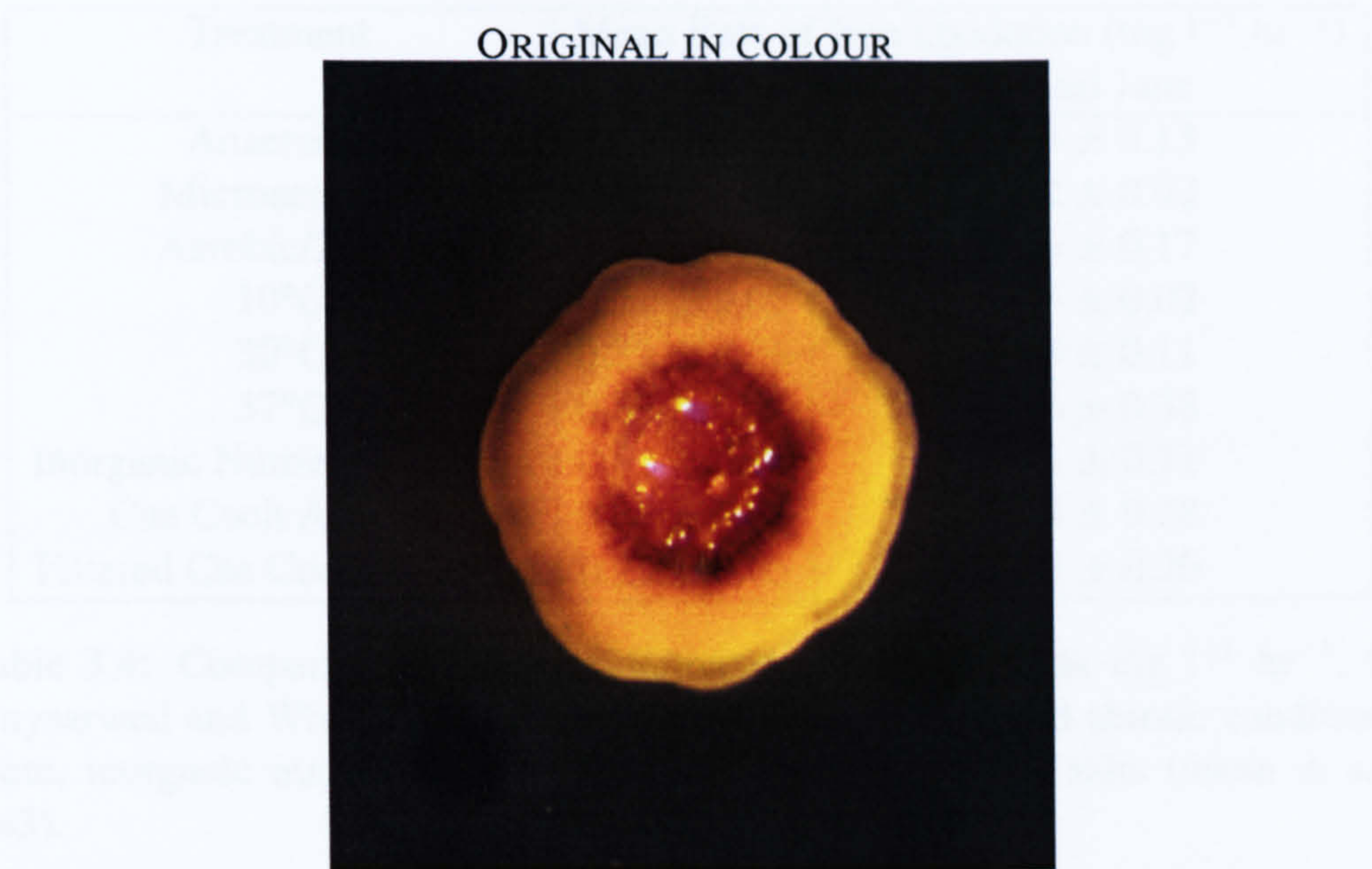
Figure 3.12: Showing the colonial morphology (x25) of isolate christened ‘Jelly’ as observed on Fe/Thio plate.
